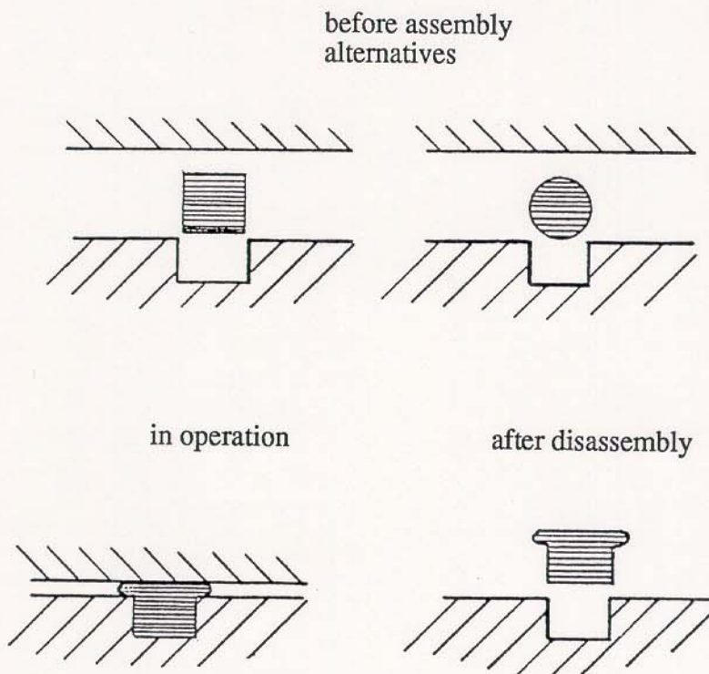
Figure 1 The gasket in principle
