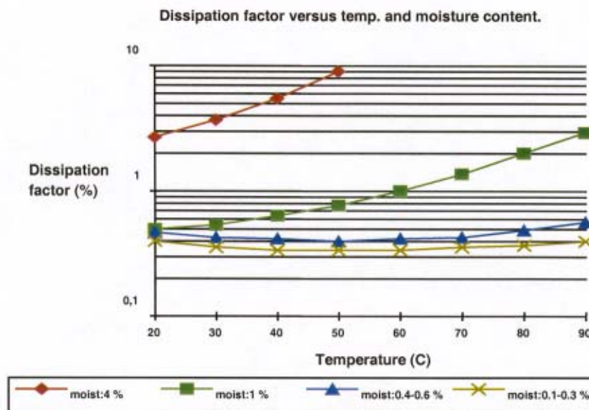
Fig. 1. \tan \delta as a function of moisture level and temperature on OIP bushings.
