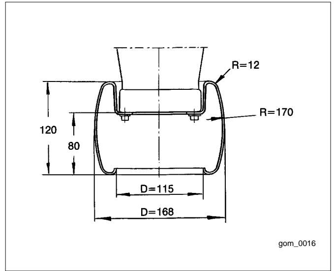
Fig. 6. End-shield.
