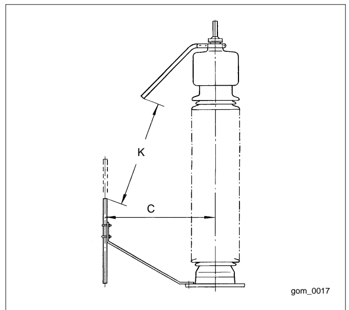
Fig. 7. Arcing horns.
