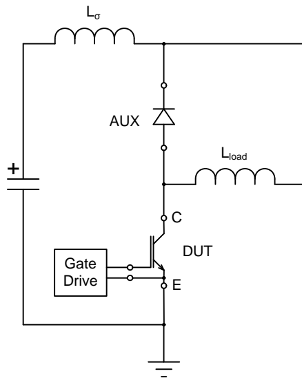
Figure 2: Electrical circuit for testing of the dynamic performance of the IGBT
