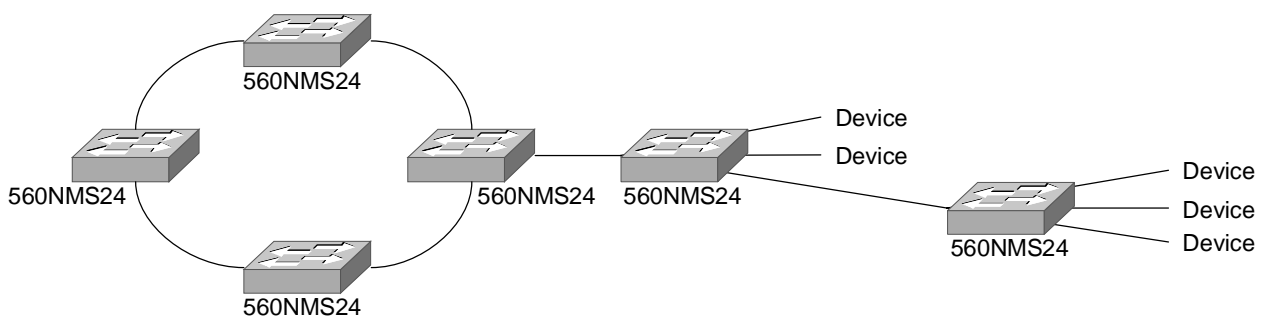
Fig. 2: Typical topology for use with 560NMS24
