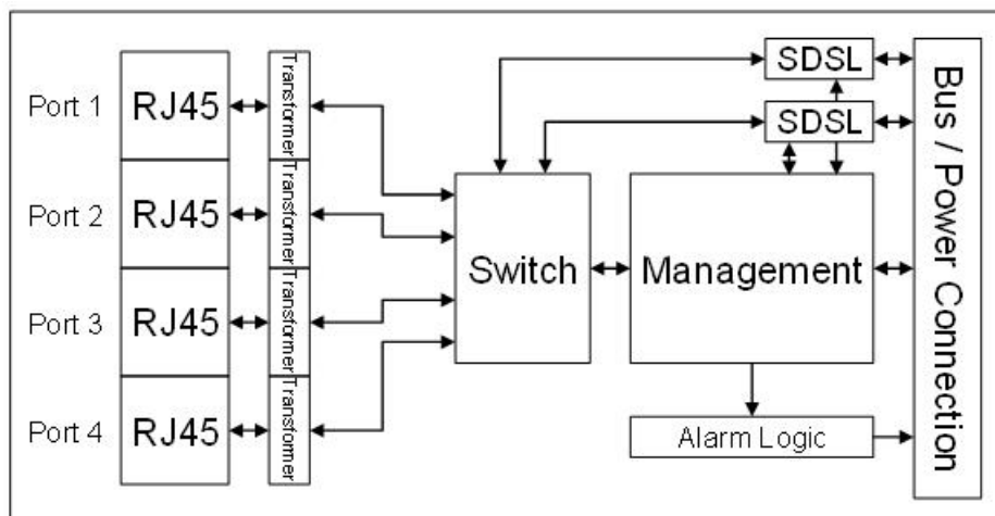
Fig. 1: Block diagram of 560NMS24
