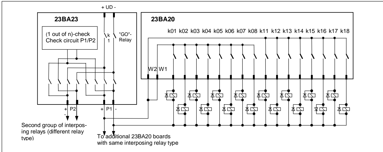
Fig. 3 :-Block diagram: Object command output with (1 out of n)-check at 1.5 pole connection
