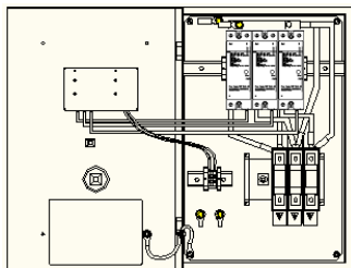
Internal layout
