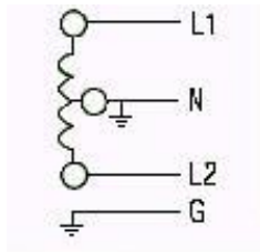
Service voltage configuration
