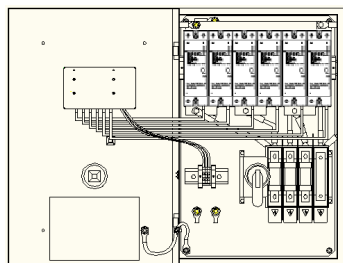
Internal layout
