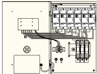
Internal layout
