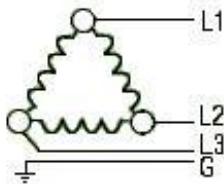
Service voltage configuration
