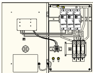
Internal layout
