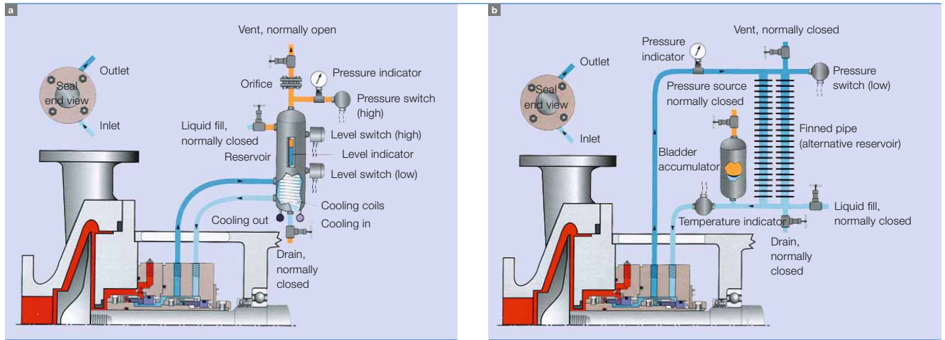
9 Actual plan the American Petroleum Institute (API) installed on pumps 11, and the new plan proposed by the API 12. Even process conditions can be changed: The pressure on the seal will be the design condition.
