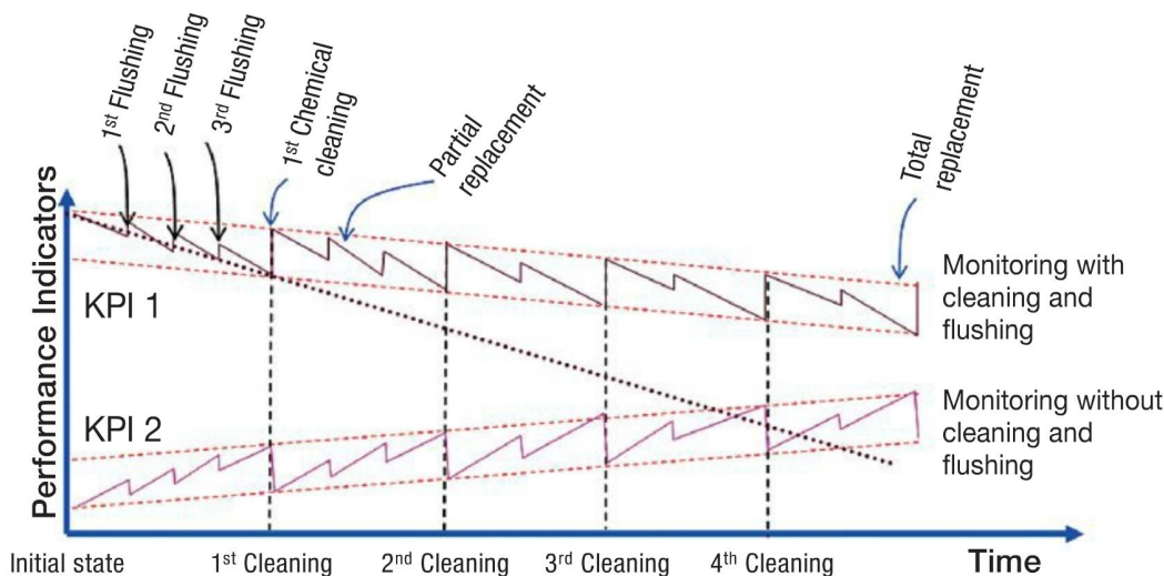
Figure 1. Performance Parameters Reflecting Dynamic Nature of Fouling
