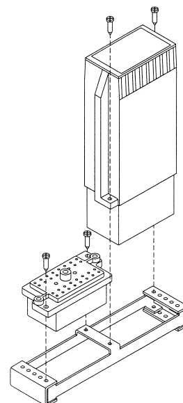
Fig. 2 The assembly of RTXP 8 and terminal base RX 1 with the 4U adapter.
