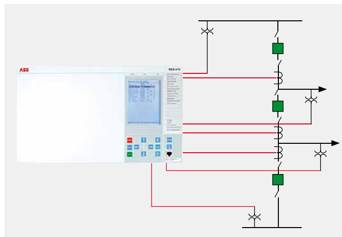
One REC670 is capable of handling control of all apparatus in one entire diameter in 1 1/2 breaker arrangement.
