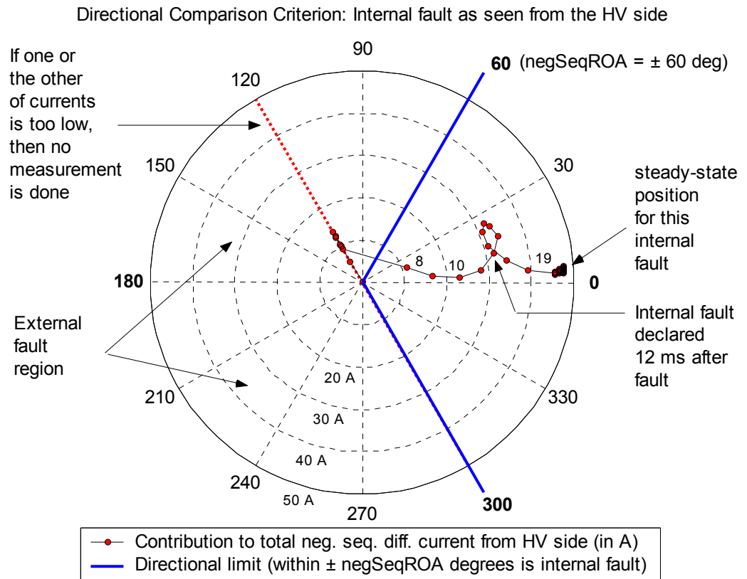
Figure 16. Operation of the internal/external fault discriminator during Tr3 autotransformer internal turn-to-turn fault
