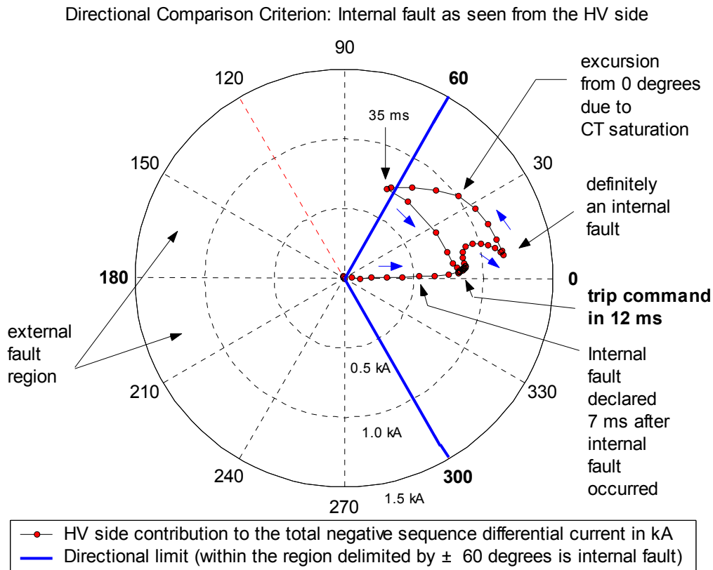
Figure 11. Operation of the internal/external fault discriminator for internal fault with CT saturation
