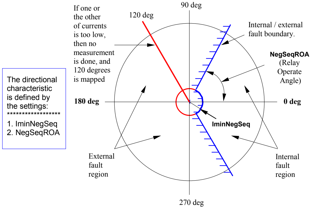
Figure 10. Operating characteristic of the internal/external fault discriminator
