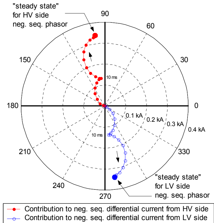
Figure 9. Trajectories of Negative Sequence Current Contributions from HV and LV sides of Yd150° power transformer during external fault
