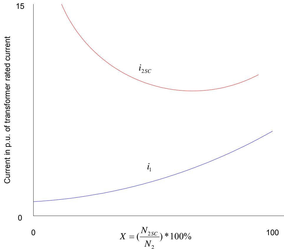
Figure 2: Inter-turn fault current vs percentage of short – circuited turns
