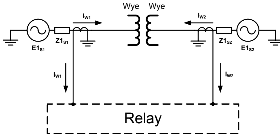
Figure 6: Used reference connections of CTs, and definition of positive direction of currents
