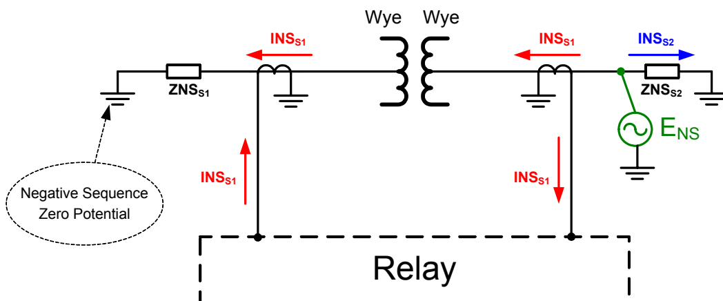
Figure 7. Flow of Negative Sequence Currents for power transformer external fault
