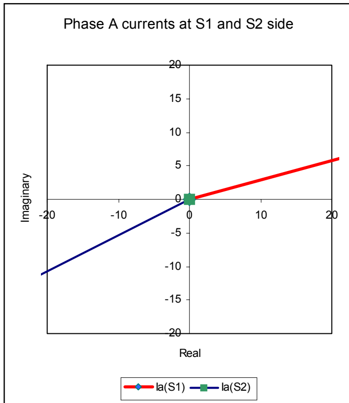
Figure 5: Angle and magnitude of phase A current at S1 and S2 side of transformer
