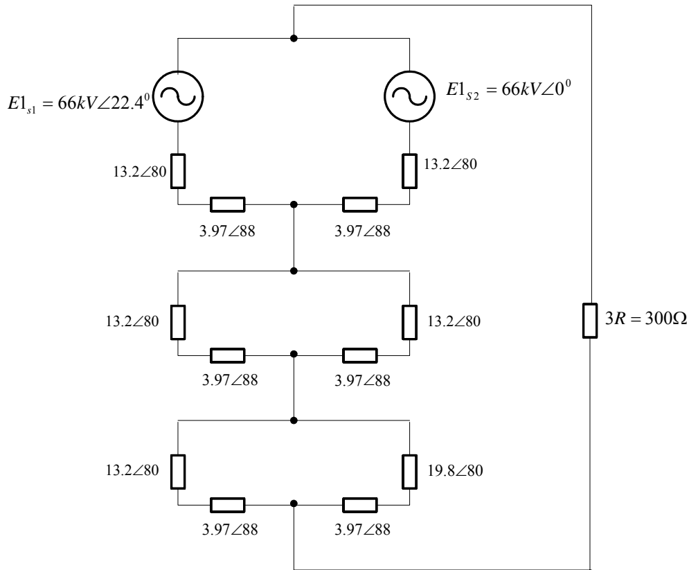
Figure 4: Sequence network for transformer internal fault
