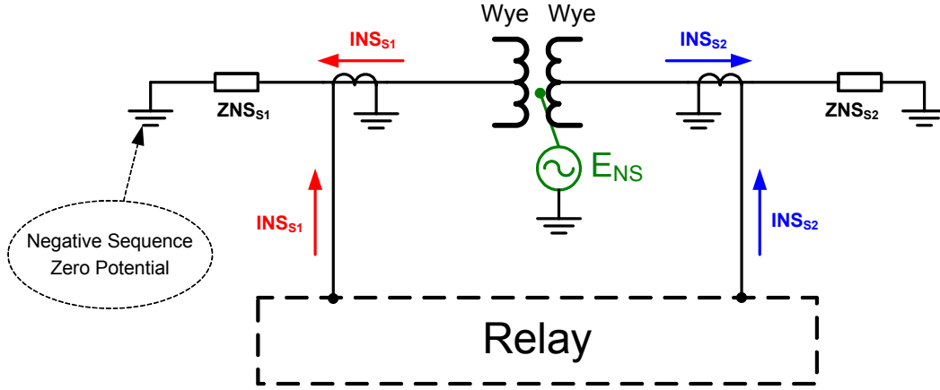
Figure 8. Flow of Negative Sequence Currents for power transformer internal fault
