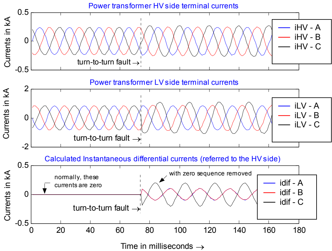
Figure 14. Measured currents from HV and LV sides, and instantaneous differential currents as calculated by traditional differential protection, during Tr3 autotransformer internal turn-to-turn fault
