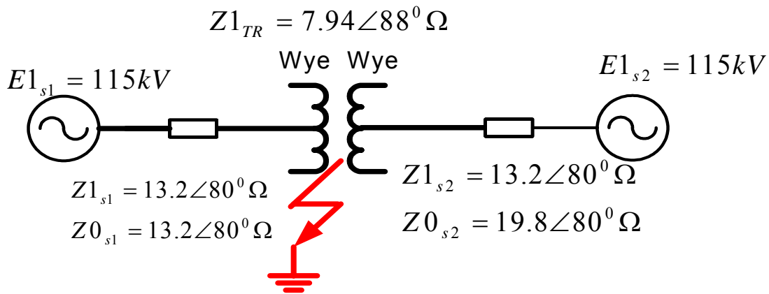
Figure 3: Two machine power system – Single Line Diagram
