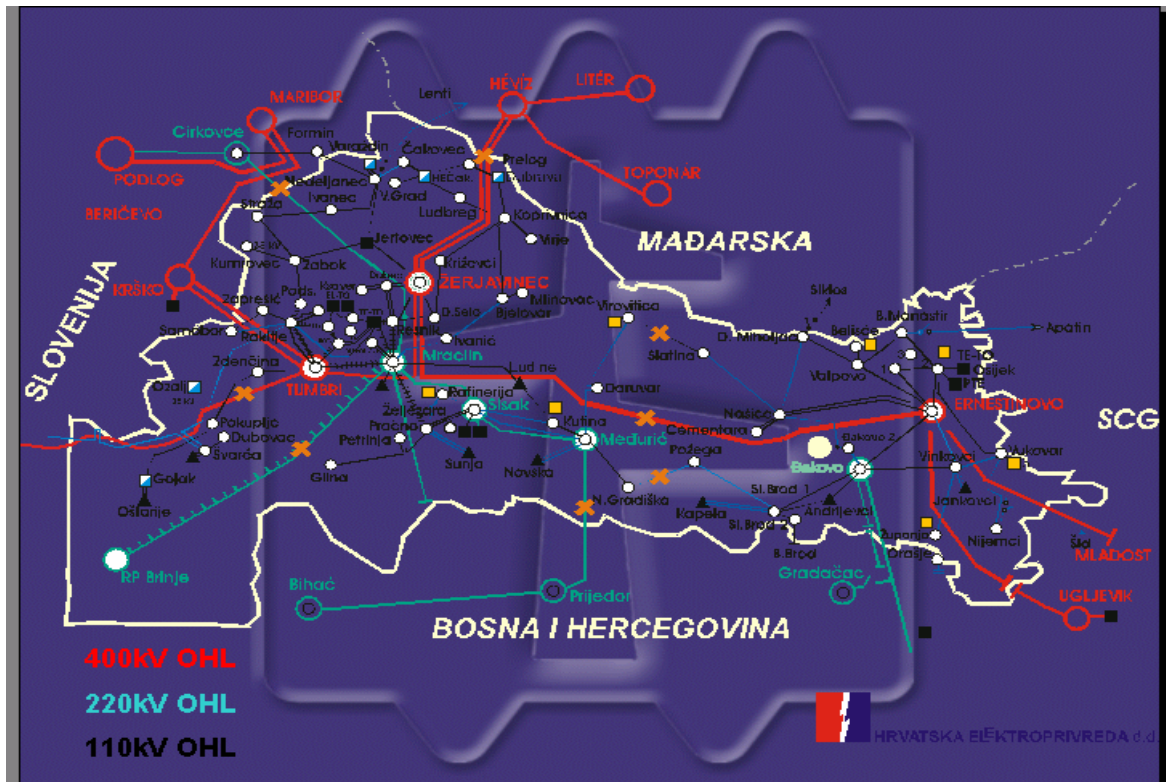
Figure 12. Part of Croatian power system grid (Courtesy of Croatian Utility – HEP)
