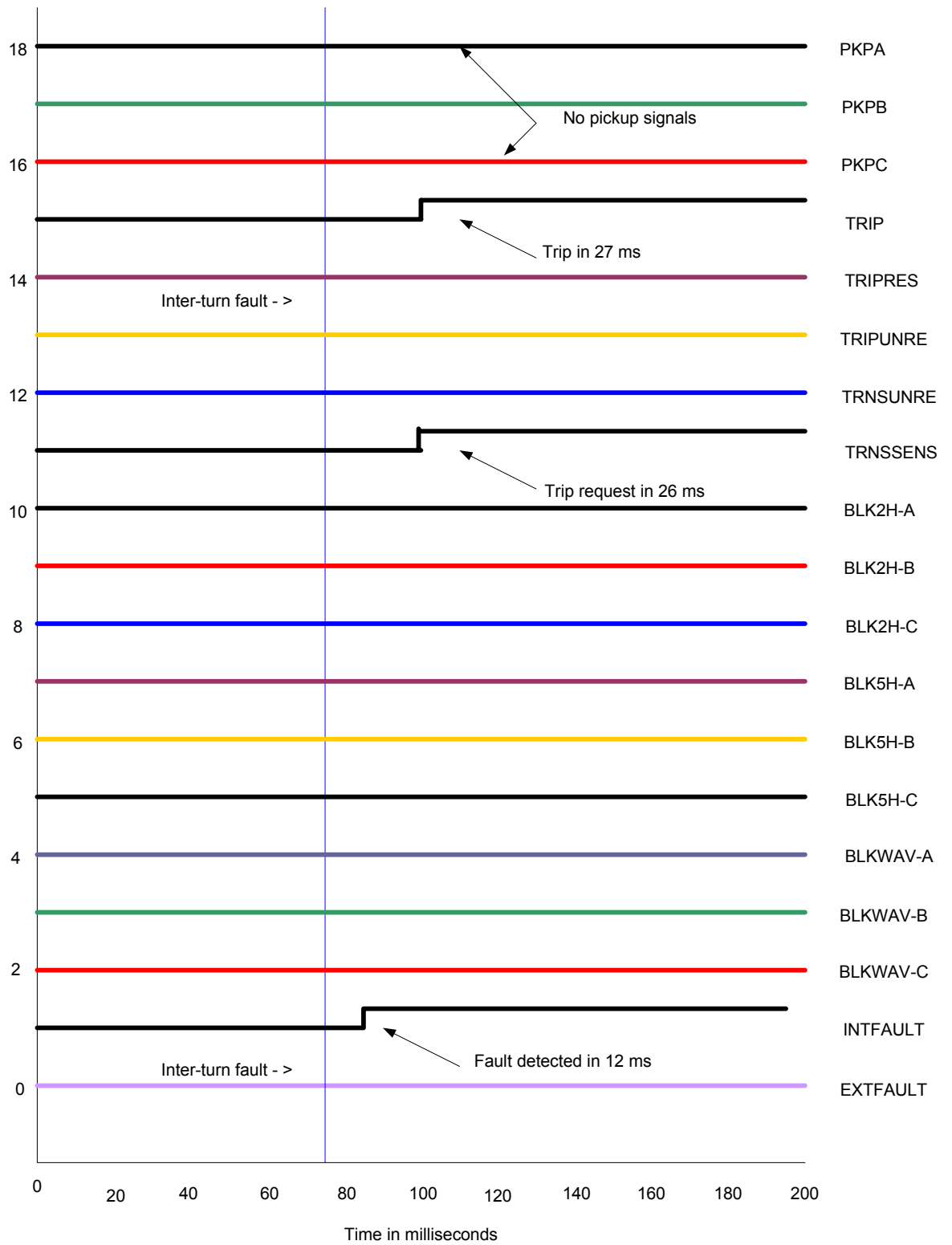
Figure 15. Output signals from new differential protection algorithm during Tr3 autotransformer internal turn-to-turn fault
