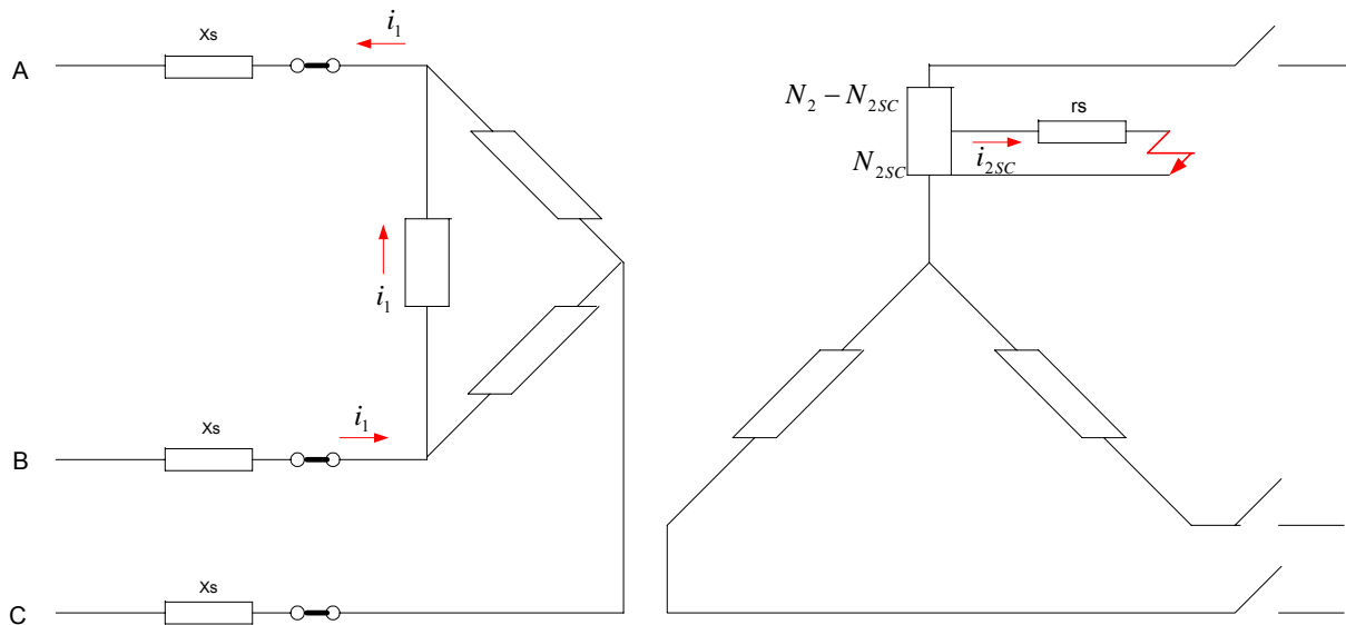
Figure 1: Inter-turn fault of transformer secondary winding
