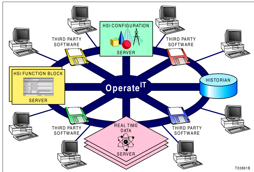
Figure 11. Software Architecture
