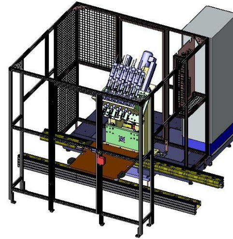
Auto/Semi-auto Assembly Station
