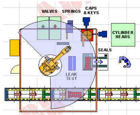
Robotic Assembly Station
