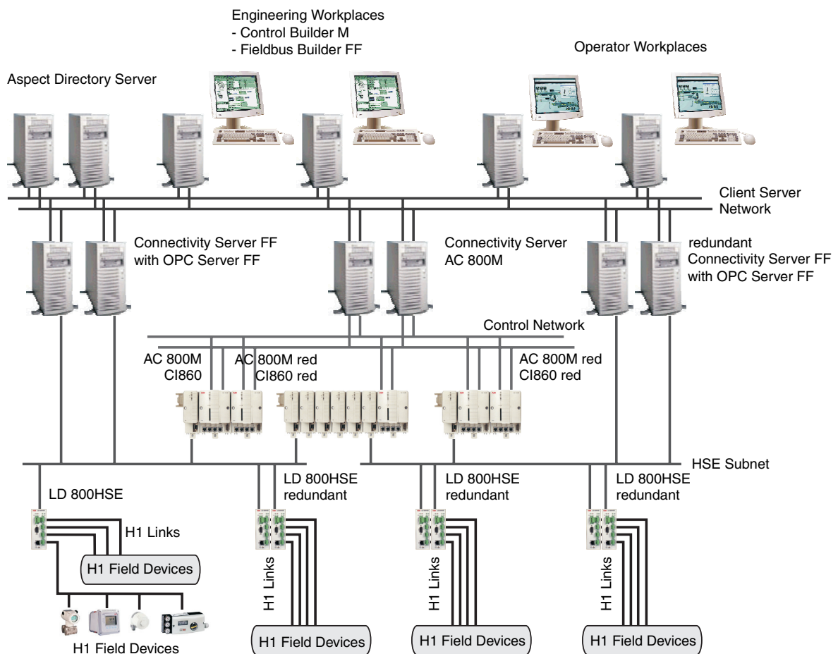
Figure 1. Sample System Structure with FF Network
