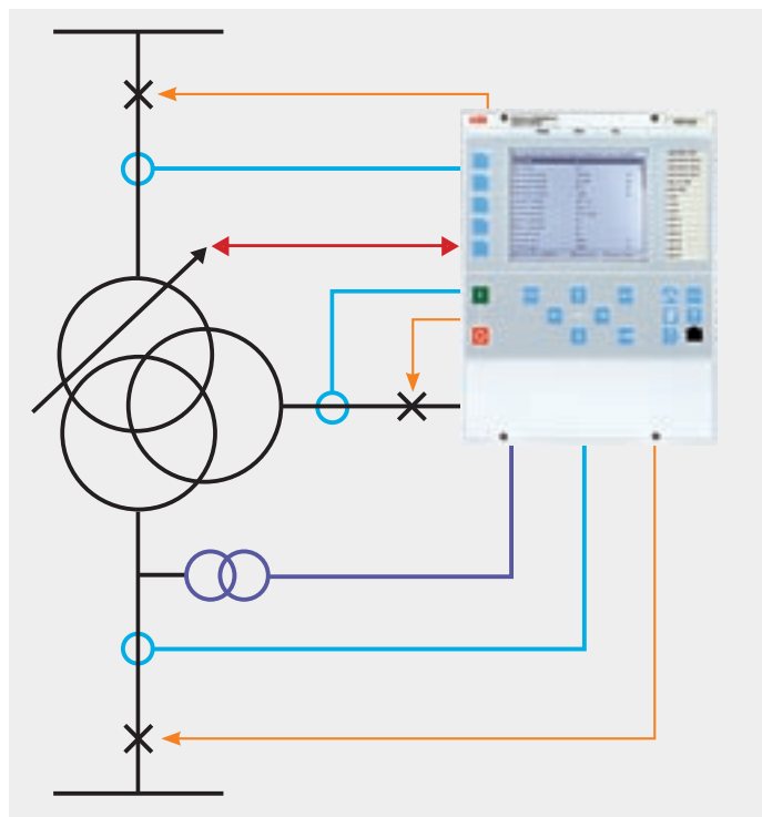
RET650 provides complete protection and control for two- and three- winding power transformers.
