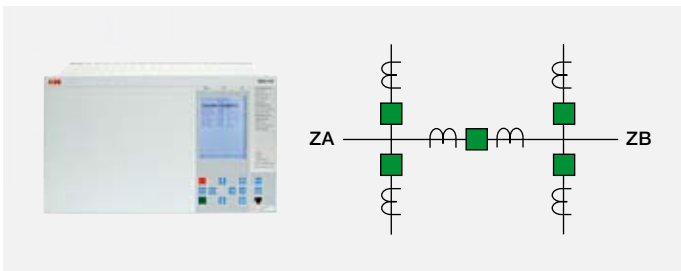
H-type station.
