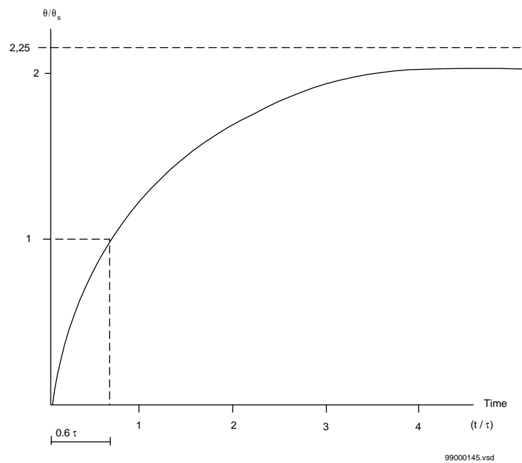
Figure 15: Temperature rise at 1.5 times rated current
