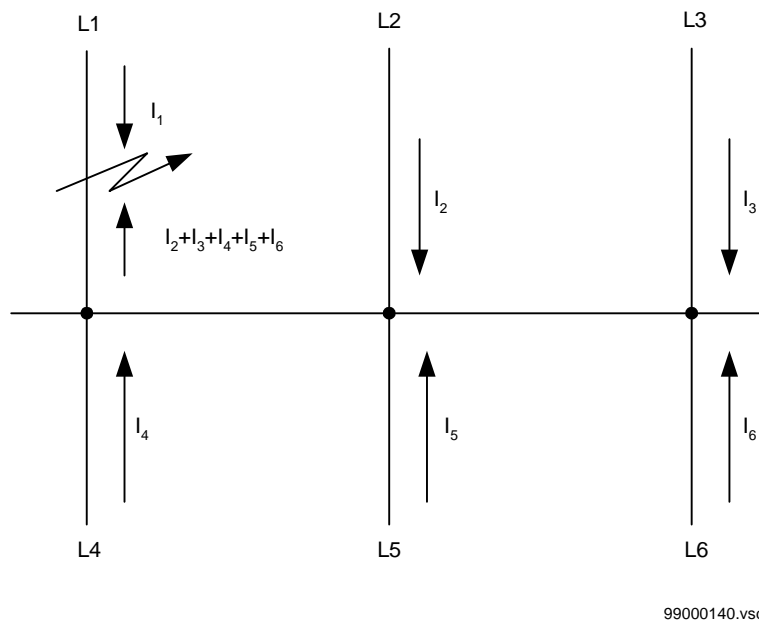
Figure 10: System with several supply circuits
