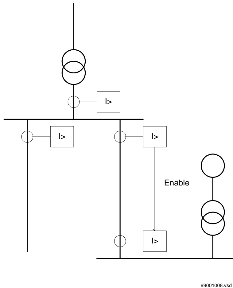
Figure 5: Example of application with enabling function
