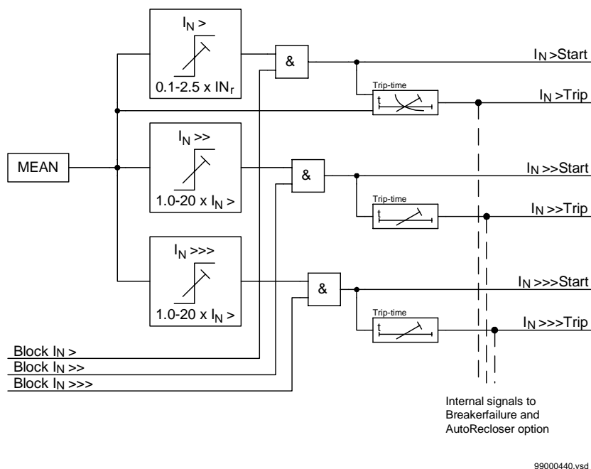
Figure 24: Simplified logic diagram for the earth-fault protection.
