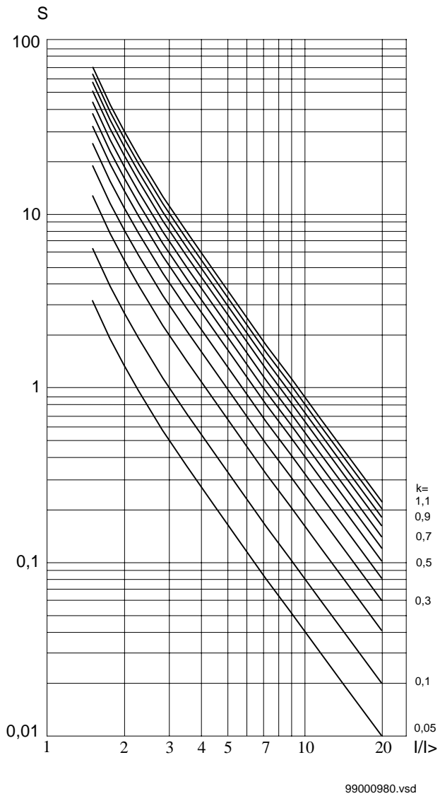
Figure 34: Extremely inverse time characteristic
