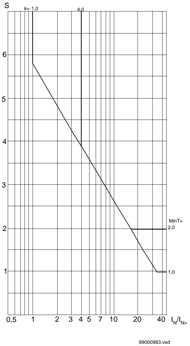
Figure 37: Logarithmic inverse time (IDG) characteristic
