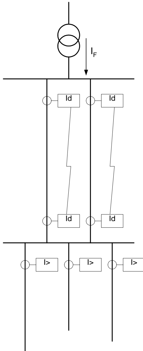
Figure 3: Radial network with a double circuit line having differential protection
