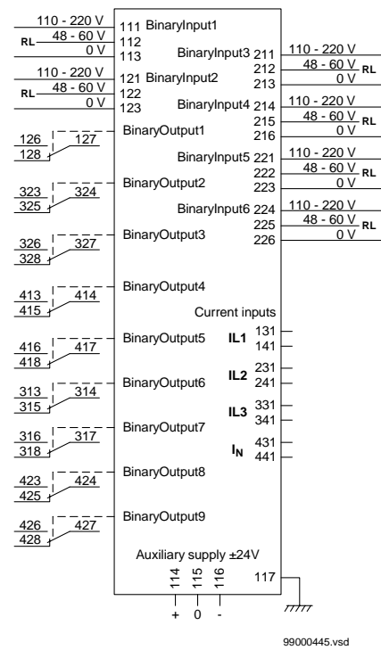
Figure 31: RXHL 411 with binary I/O module
