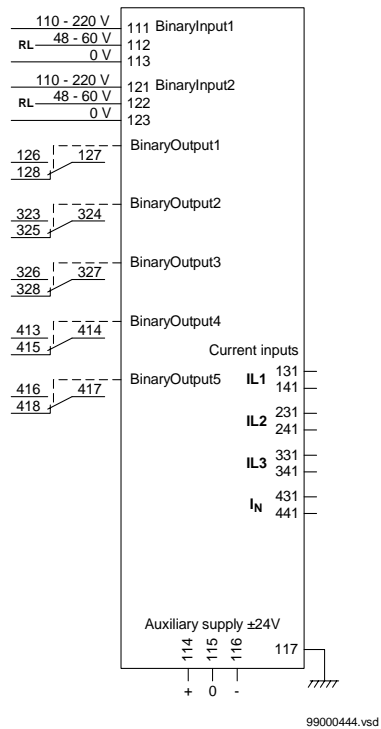
Figure 30: RXHL 411 basic version
