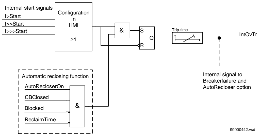
Figure 26: Simplified logic diagram for the intentional overreach trip function.
