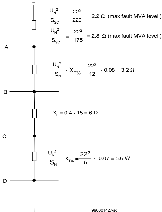
Figure 12: Equivalent impedance network
