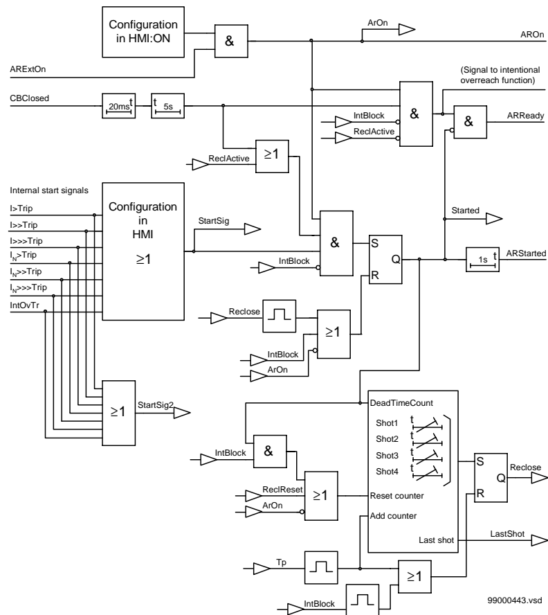
Figure 27: Simplified logic diagram for the automatic reclosing function, part 1.
