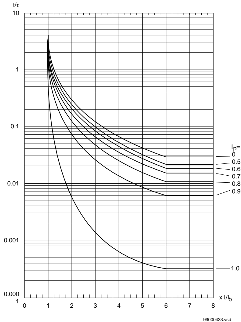
Figure 16: Operate time curves of the thermal protection
