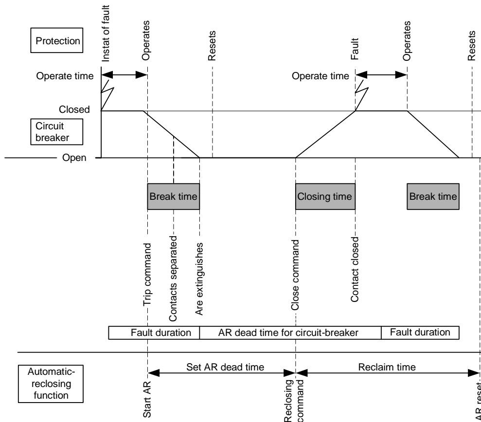
Figure 18: Single-shot automatic reclosing at a permanent fault
