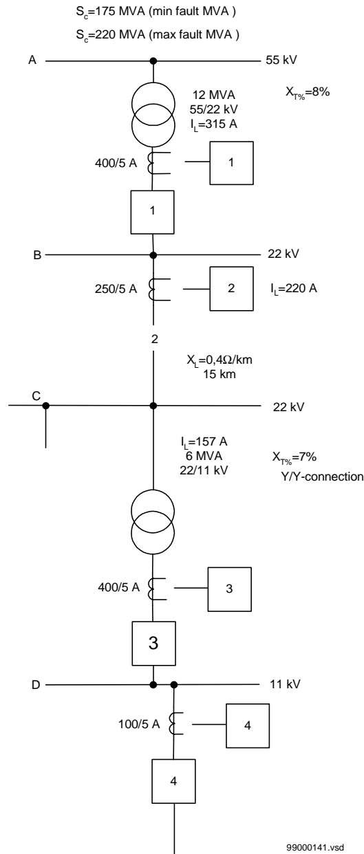
Figure 11: Radial network
