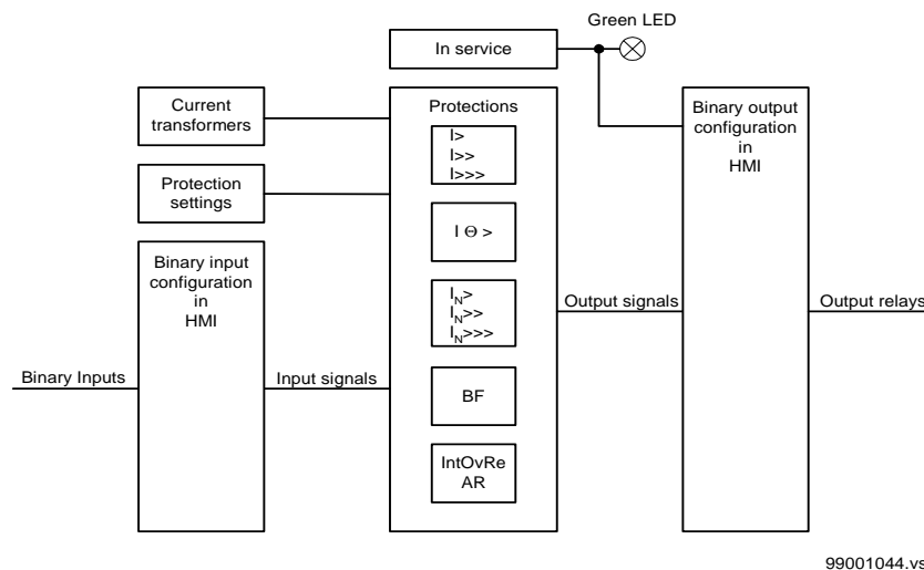
Figure 20: Simplified logic diagram for the compact current relay RXHL 411.
