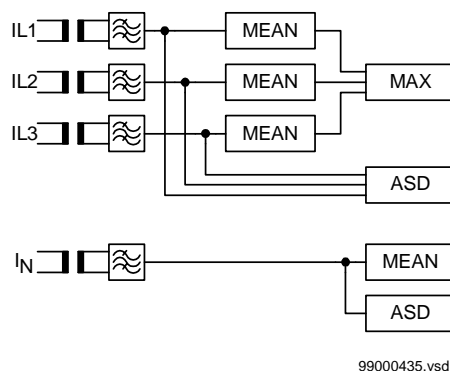
Figure 21: Calculated values from the input signals
