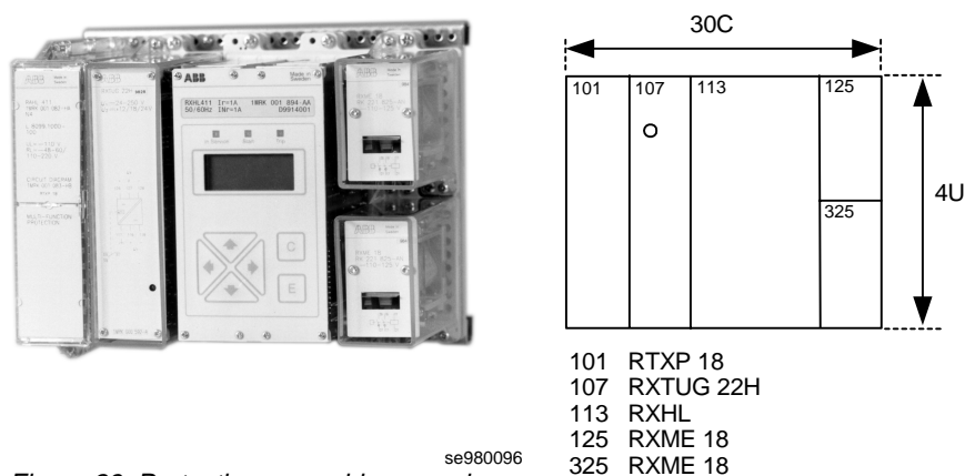
se980096 Figure 29: Protection assembly example
