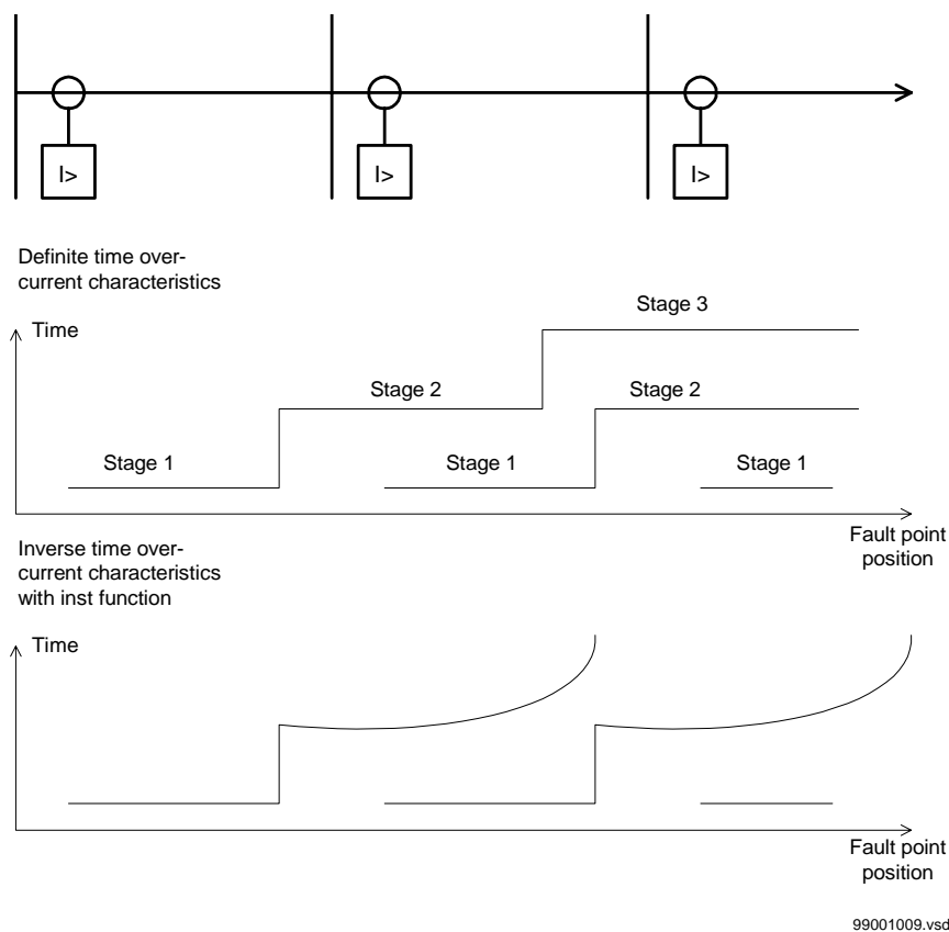
Figure 6: Fault time as a function of fault position in a radial network with overcurrent protection
