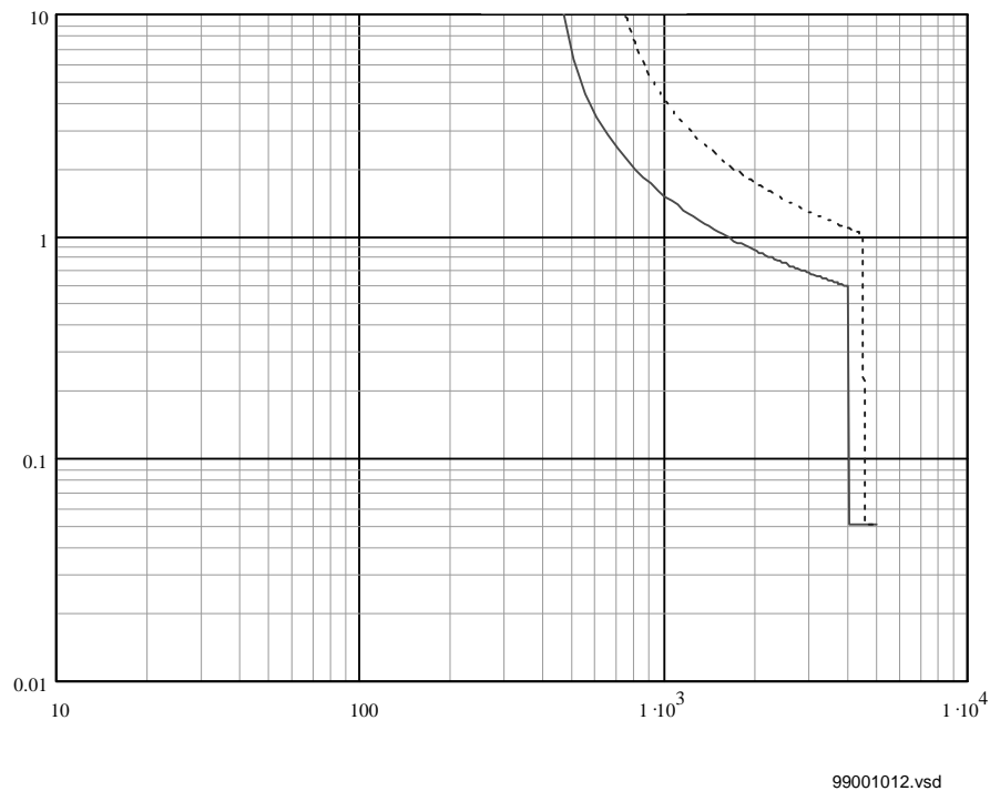
Figure 9: Example of time-current selectivity curves
