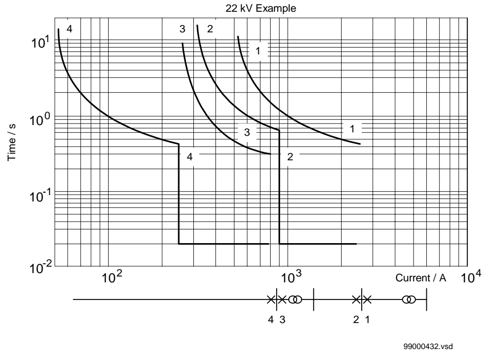
Figure 13: Current-time characteristics for the studied network
