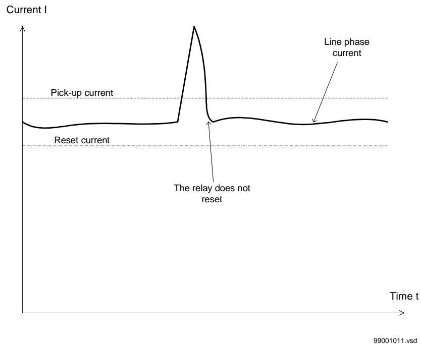
Figure 8: Clarification of reset current of overcurrent protection
