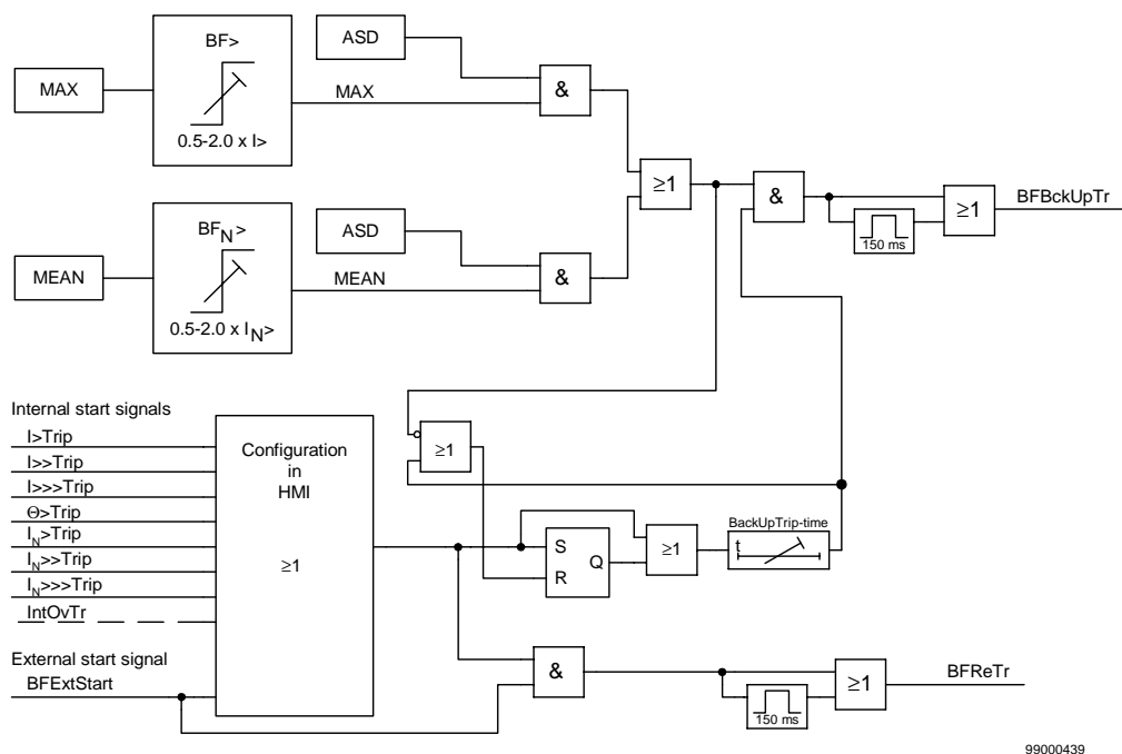
Figure 25: Simplified logic diagram for the breaker-failure protection.
