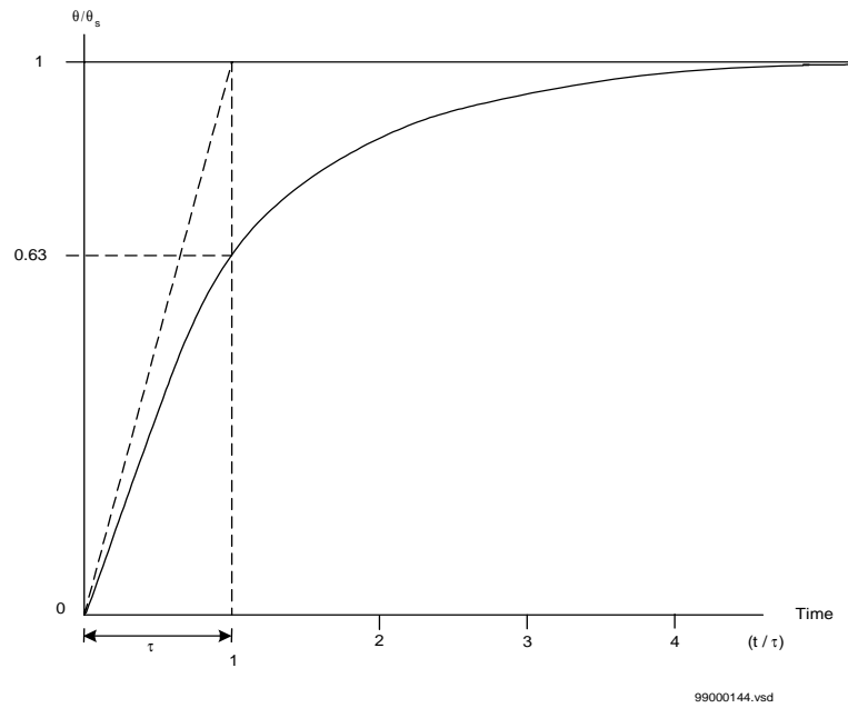
Figure 14: Temperature rise at rated current
