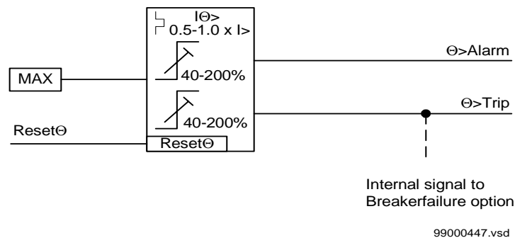
Figure 23: Simplified logic diagram for the thermal overload protection
