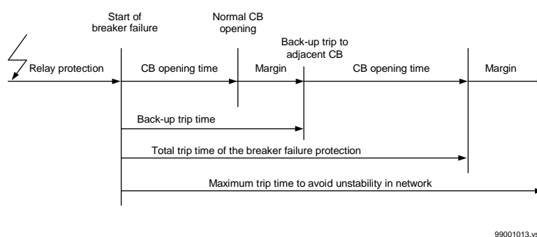
Figure 17: Operating diagram for back-up trip at a breaker-failure situation.
