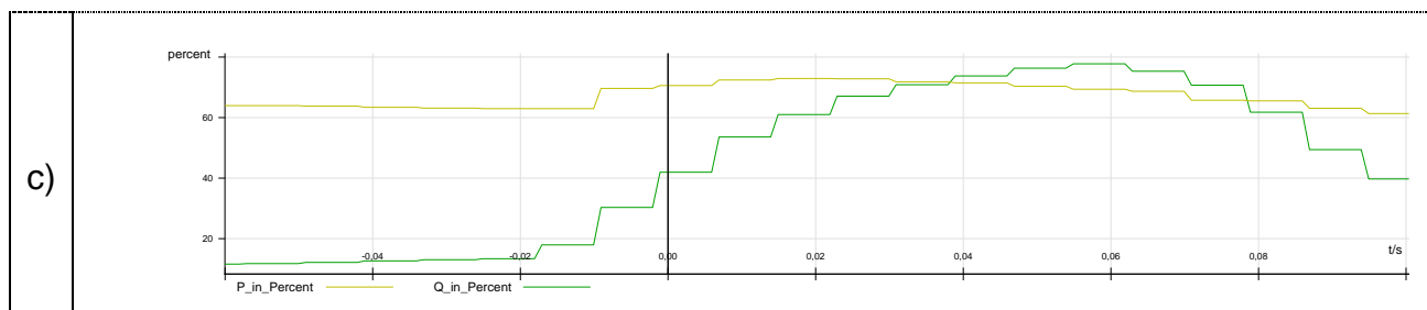
Fig. 12: External fault in generator mode ( P=+63.9\% , Q=+11.8\% before the fault)
