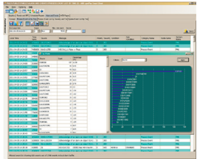
Process event list by time: In this event list, an overlapping window also shows the number of events per object (as a bar chart) and as a percentage of the total events. This information lets you analyze events directly in the list and identify which objects to prioritize in order to reduce the total number of process events.
