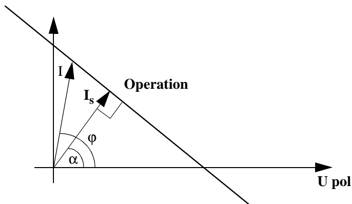
Fig. 11 Function characteristic of the RXPDK 21H relay.
