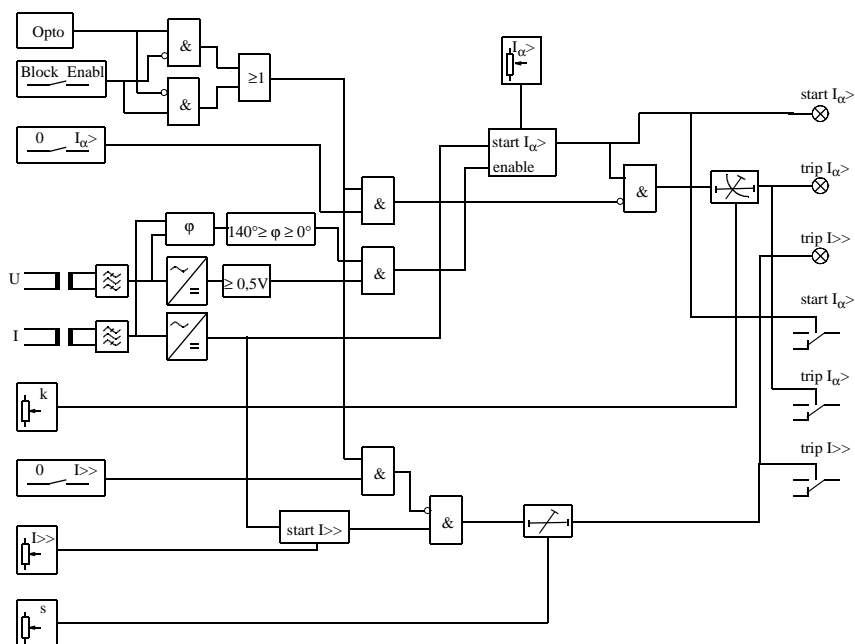
Fig. 18 Simplified diagram of the RXPDK 23H relay
