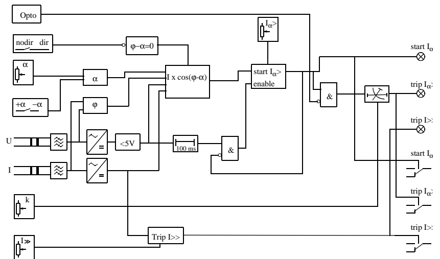
Fig. 12 Simplified functional diagram of the RXPDK 21H relay
