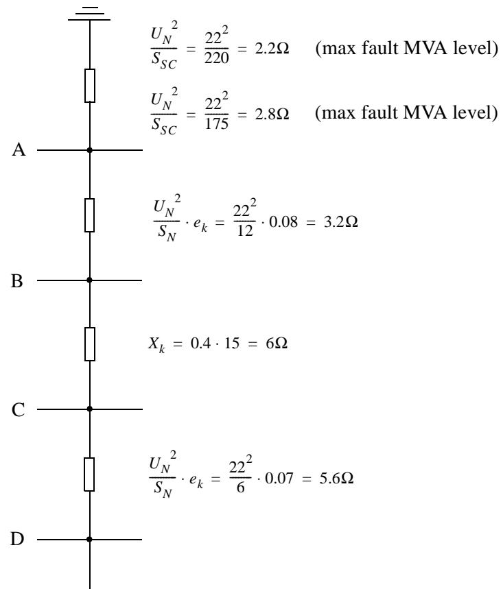
Fig. 5 Equivalent impedance network
