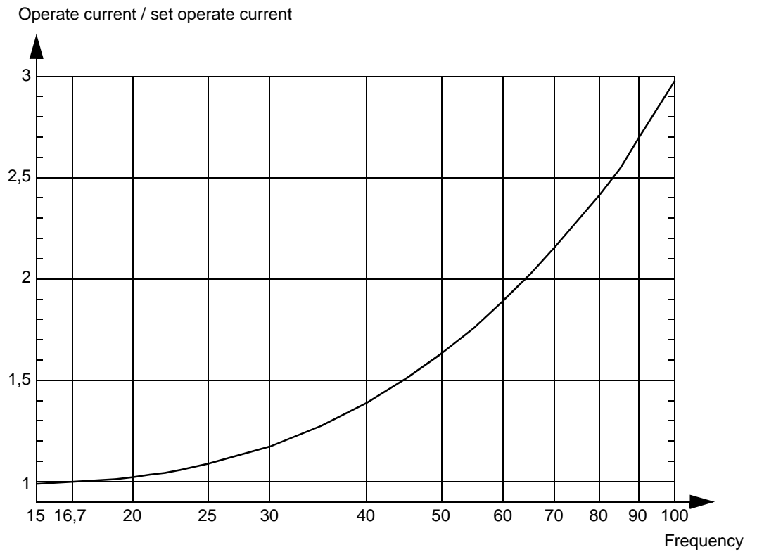
Fig. 33 Typical frequency characteristic for RXIDK 16 2/3 Hz, valid for I \leq 65 \times I_s
