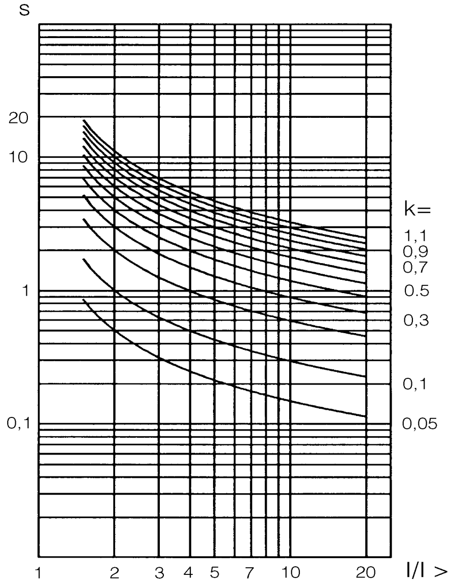
Fig. 35 Normal inverse characteristic
