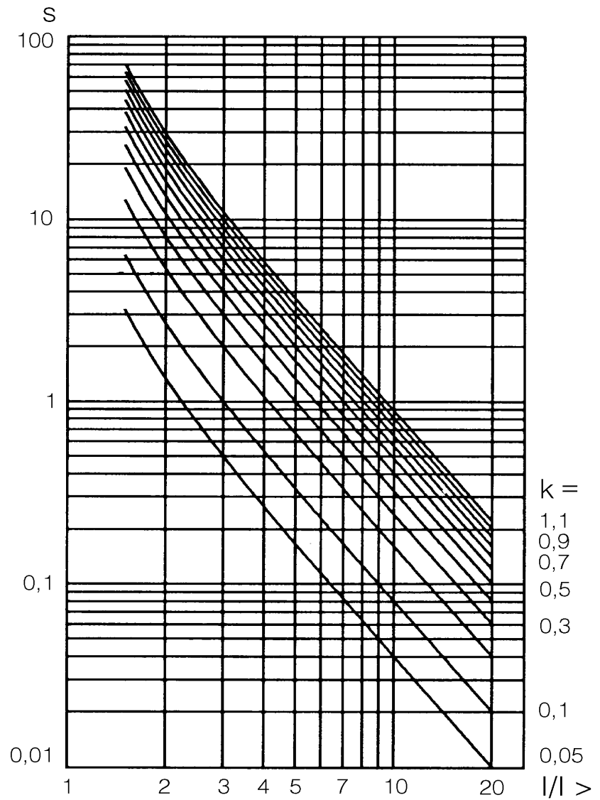
Fig. 37 Extremely inverse characteristic
