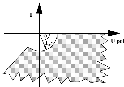
Fig. 17 Function characteristics for the RXPDK 23H I_{\alpha>} function.
