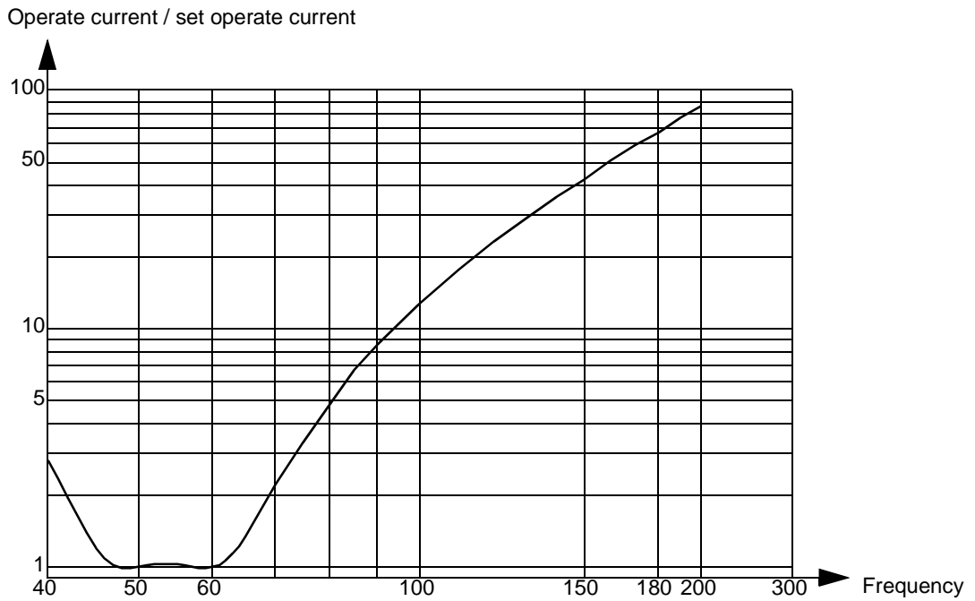
Fig. 30 Typical frequency characteristic for RXIDK 50-60 Hz, sharp, valid for I \leq 65 \times I_s
