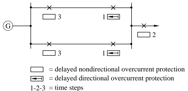
Fig. 2 Radially supplied system with parallel lines
