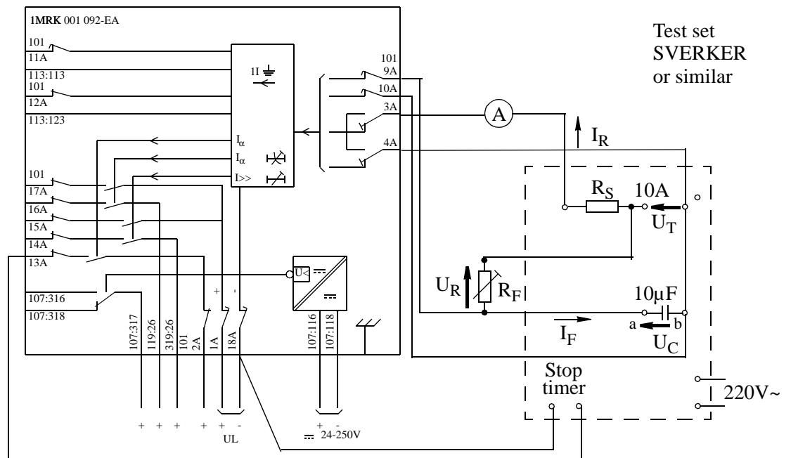
Fig. 49 Connection of test apparatus to earth fault prot. RAPDK 231
