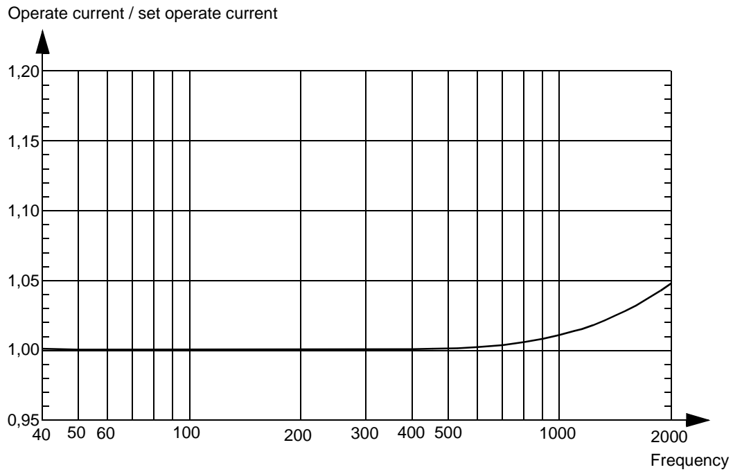
Fig. 32 Typical frequency characteristic for RXIDK 40-2000 Hz, valid for I \leq 65 \times I_s
