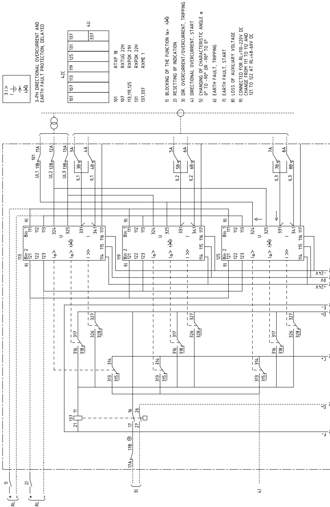
Fig. 57 Circuit diagram 1MRK 001 062-VB, Page 1
