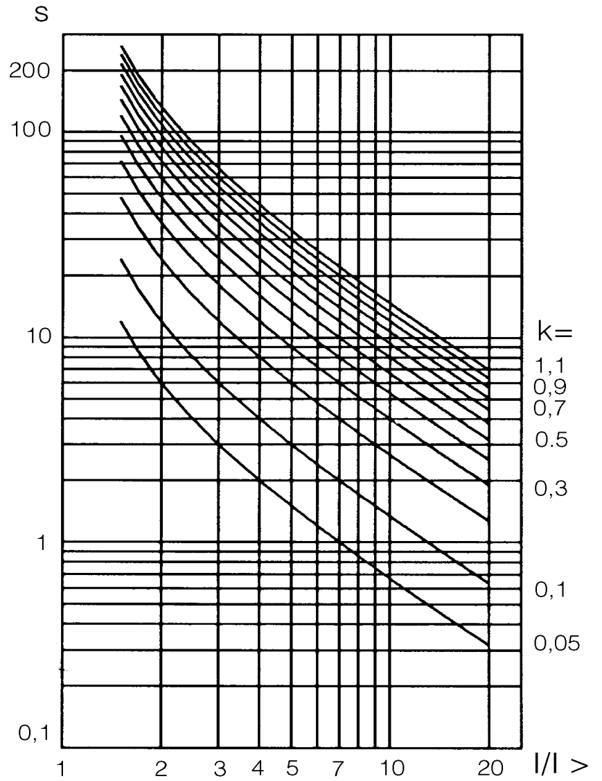
Fig. 38 Long-time inverse characteristic
