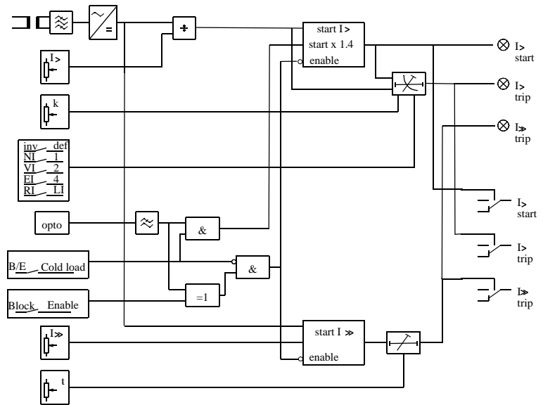
Fig. 9 Simplified functional diagram of the RXIDK 2H relay
