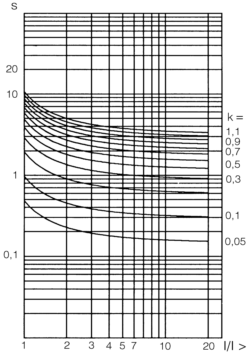
Fig. 39 RI inverse characteristic
