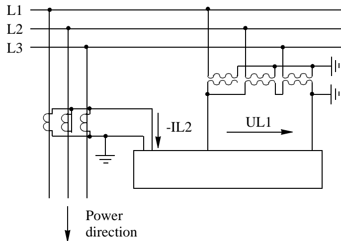
Fig. 52 Directional testing of earth-fault relay with characteristic angle \alpha = -90^\circ
