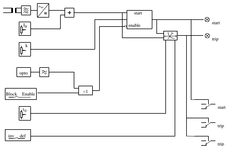
Fig. 10 Simplified functional diagram of the RXIDG 21H relay
