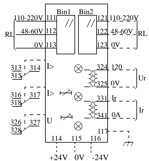
Fig. 26 Terminal diagram RXPDK 22H
