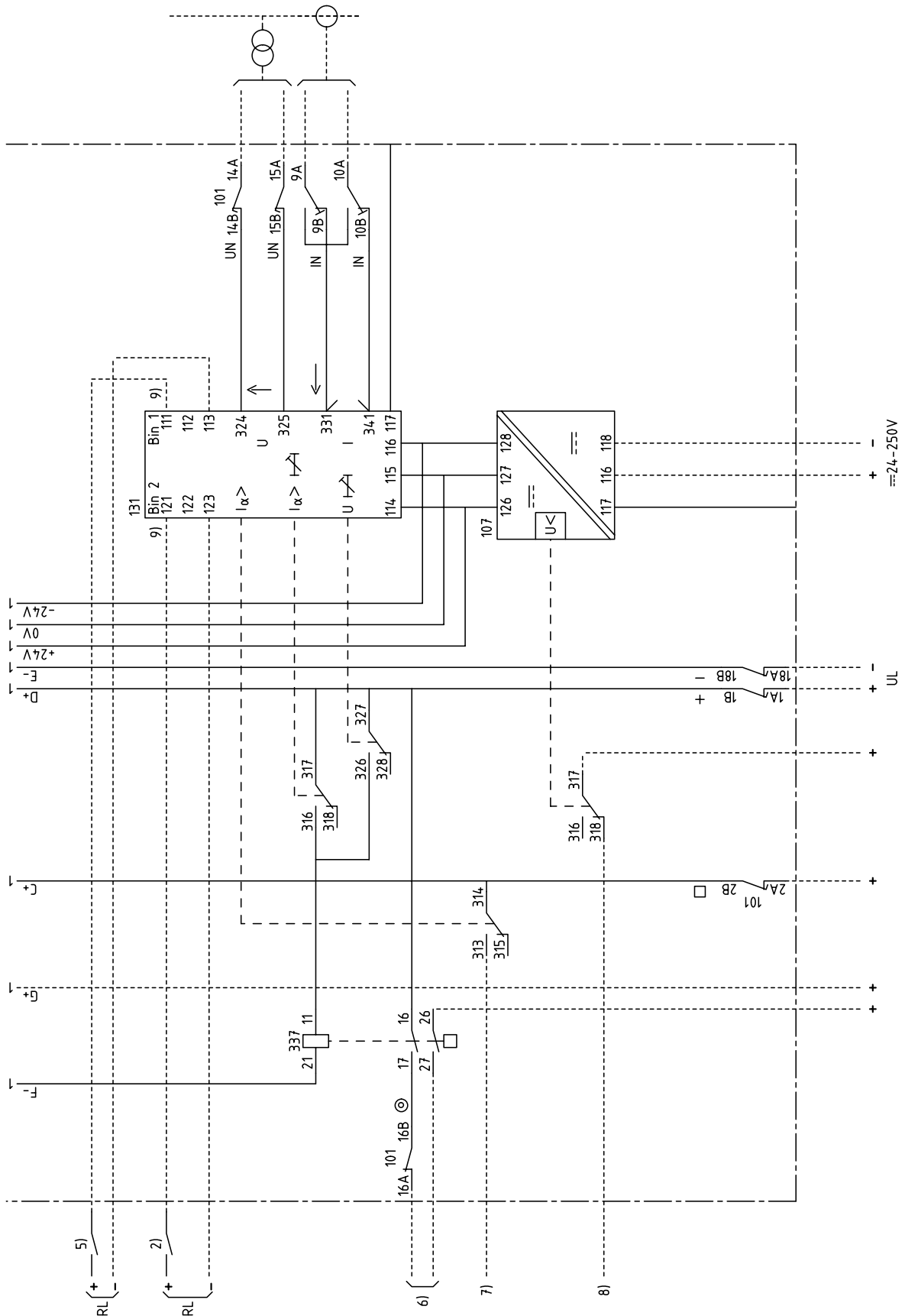
Fig. 58 Circuit diagram 1MRK 001 062-VB, Page 2
