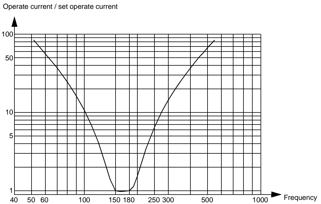
Fig. 31 Typical frequency characteristic for RXIDK 150-180 Hz, sharp, valid for I \leq 65 \times I_s
