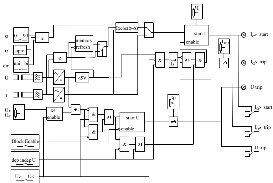
Fig. 15 Simplified functional diagram of the RXPDK 22H relay
