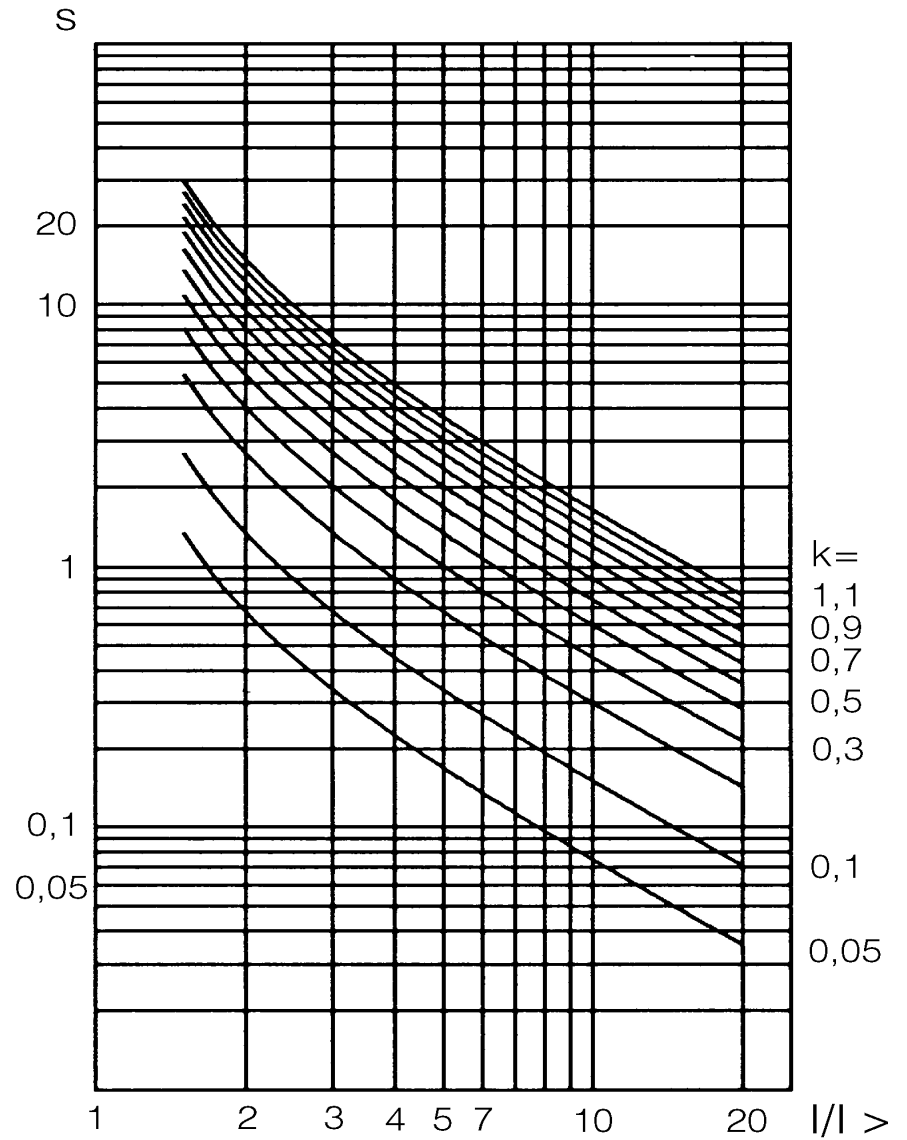
Fig. 36 Very inverse characteristic
