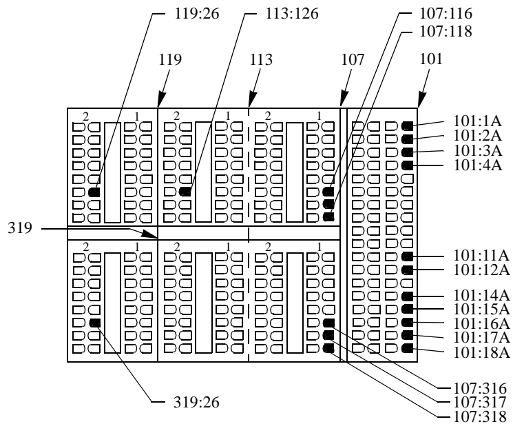
Fig. 46 Location of the terminals shown on diagram 1MRK 001 003-EAA
