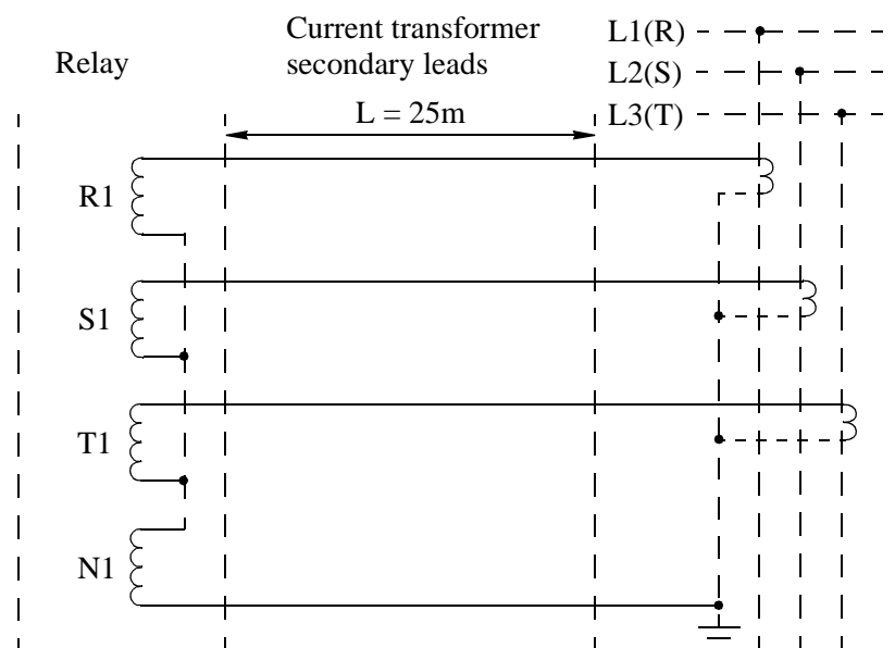
Fig. 7 Equivalent circuit for current transformer to earth-fault relay.
