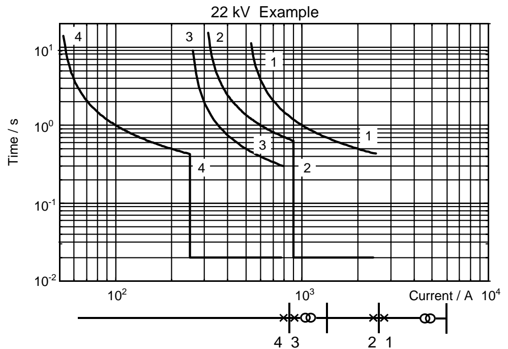
Fig. 6 Current-time characteristics for the studied network
