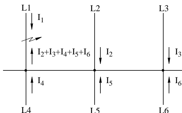
Fig. 3 System with several supply circuits
