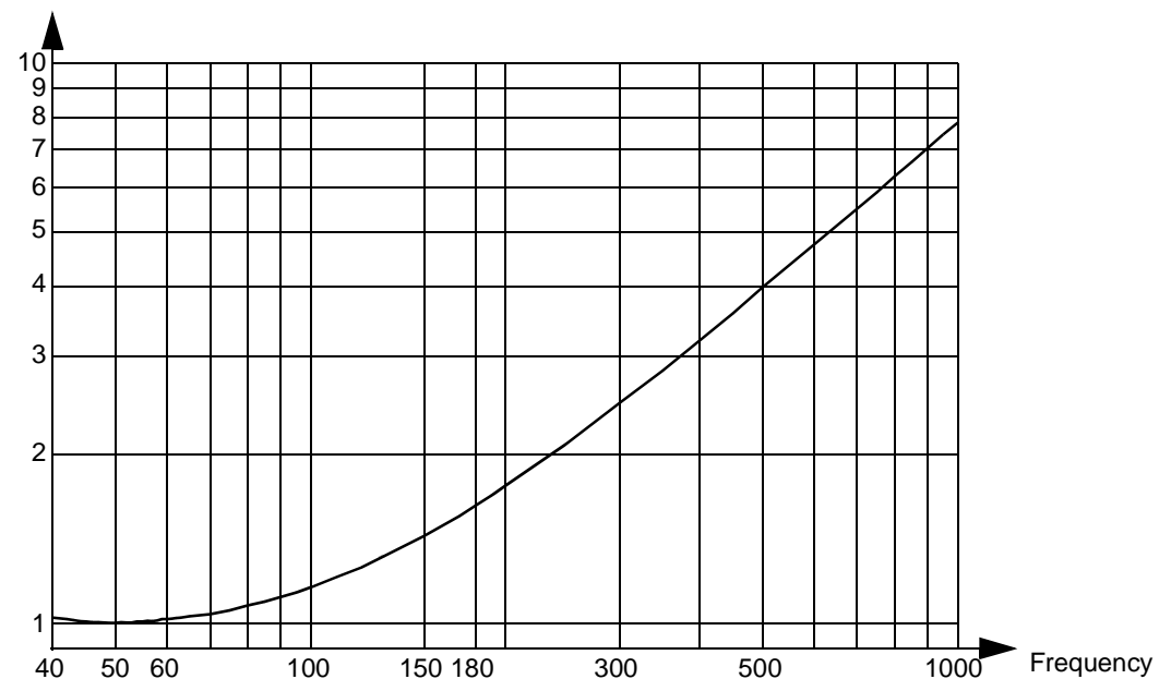
Fig. 29 Typical frequency characteristic for RXIDK 50-60 Hz, standard, valid for I \leq 65 \times I_s
