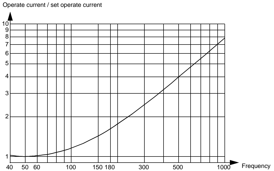
Fig. 34 Typical frequency characteristic for RXIDG 50-60 Hz, valid for valid for I \leq 100 \times I_s
