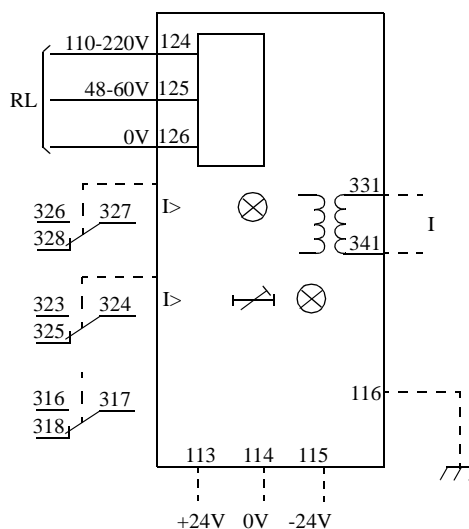
Fig. 22 Terminal diagram RXIDG 21H
