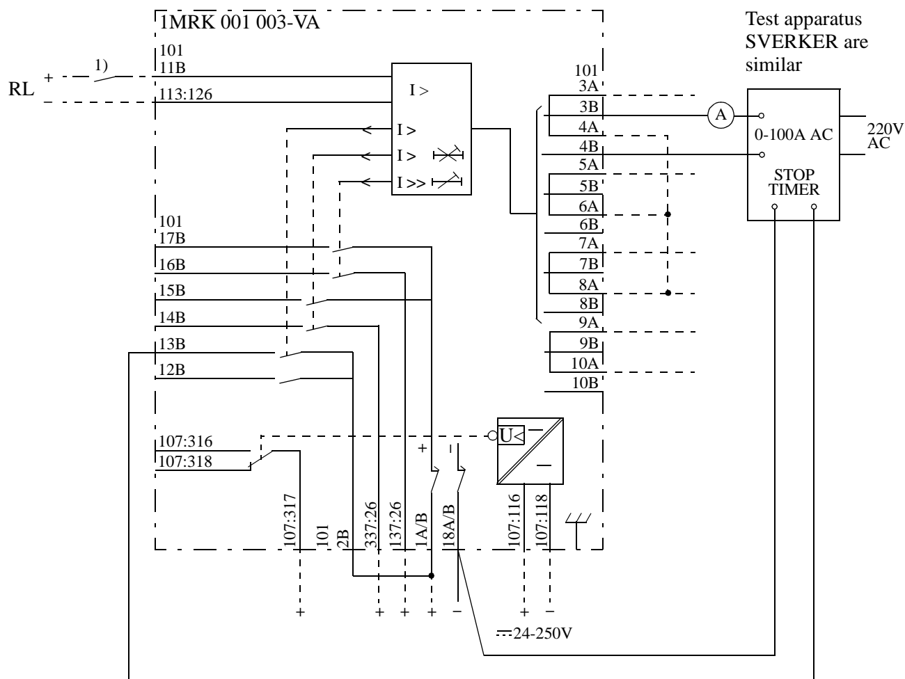
Fig. 47 Connection of test apparatus for testing of phase L1
