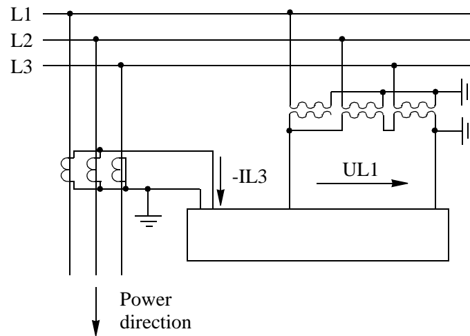
Fig. 51 Directional testing of earth-fault relay with characteristic angle \alpha = 0 to +90^\circ
