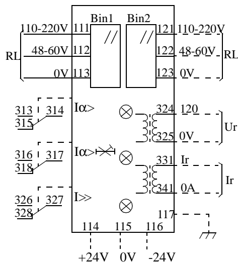
Fig. 24 Terminal diagram RXPDK 21H
