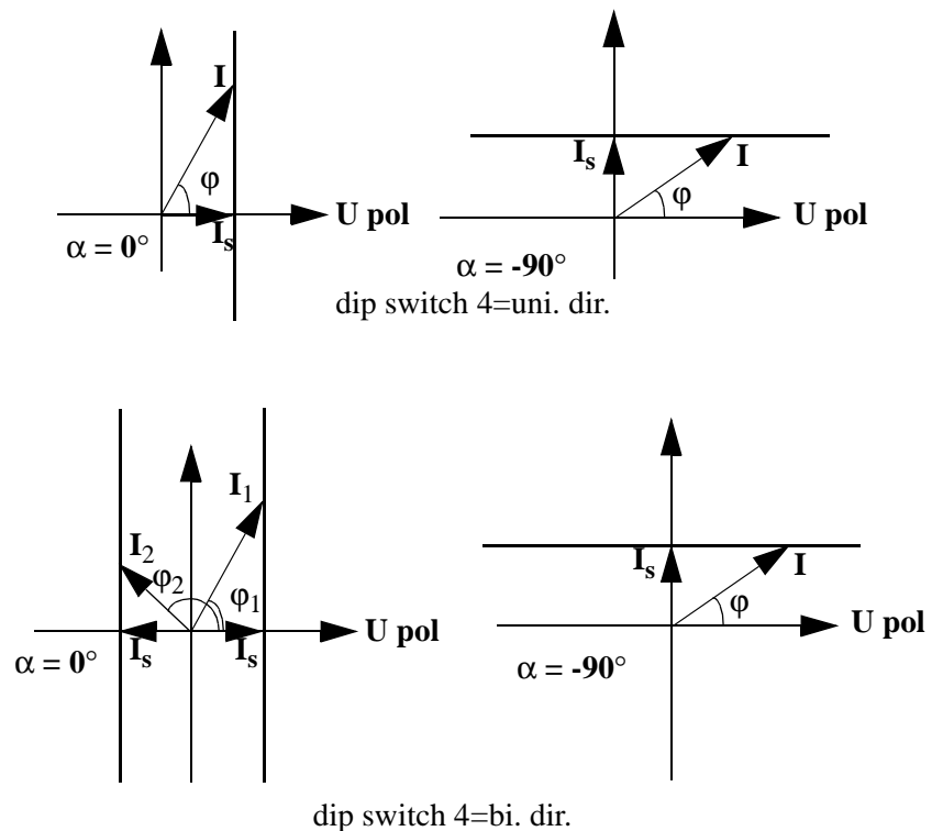
Fig. 16 Function characteristics for the RXPDK 22H relay
