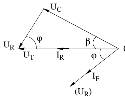
Fig. 48 Testing of directional relay RXPDK 21H with positive characteristic angle \alpha . Principle diagram
