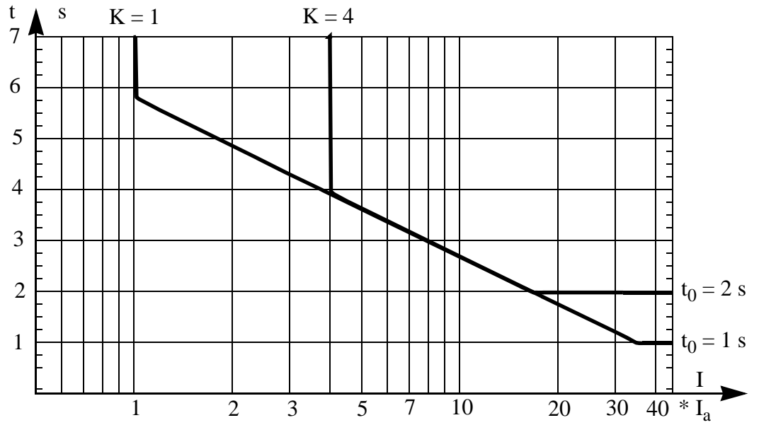
Fig. 40 Logarithmic inverse characteristic
