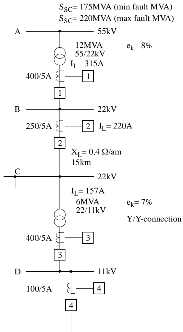
Fig. 4 Radial network
