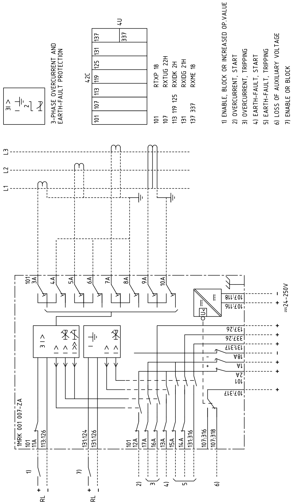
Fig. 64 Terminal diagram 1MRK 001 007-ZAA
