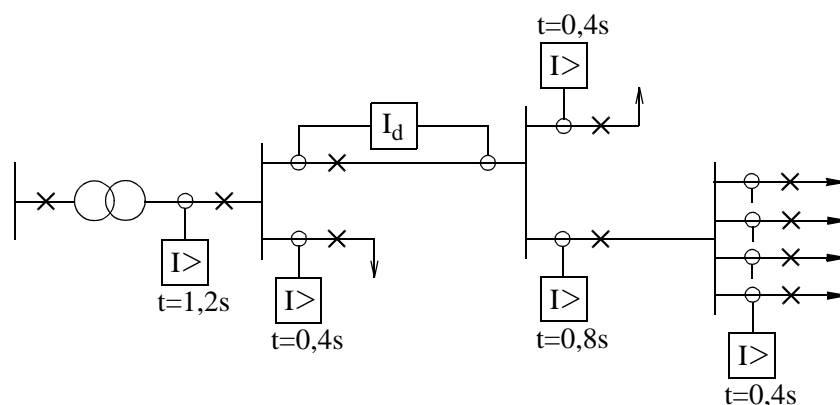
Fig. 1 Example showing how a longitudinal differential protection can reduce the number of selective steps
