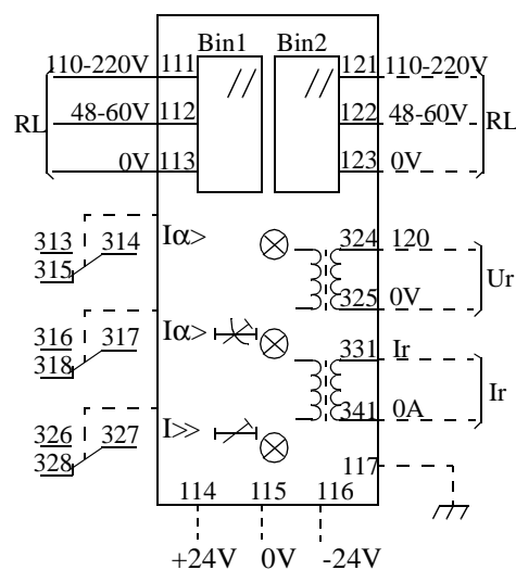
Fig. 28 Terminal diagram RXPDK 23H
